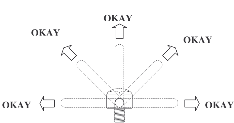
Swivel Hoist Ring - same load rating at any angle
