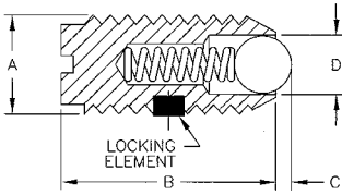
Ball Plunger
