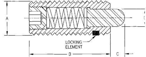
Spring Plunger
